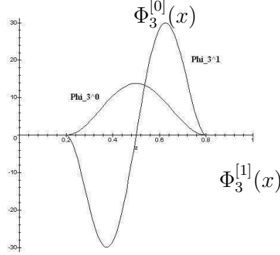
Figure 2: Shape functions
